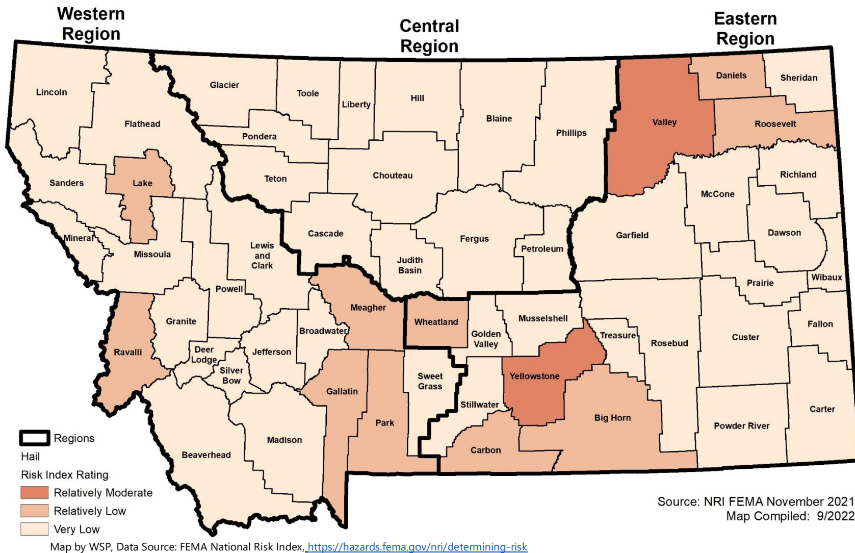
Figure 4-53 NRI Risk Index Rating for Hail
