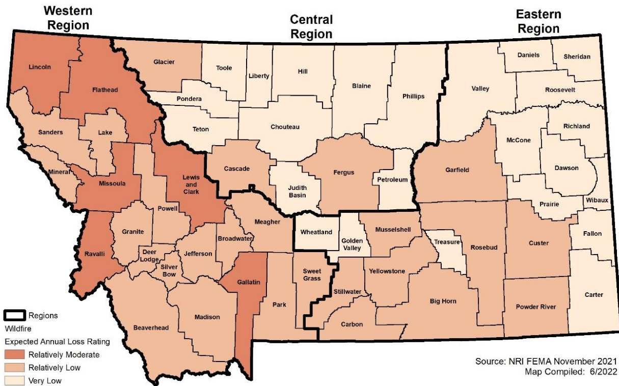
Figure 4-109 NRI Wildfire Expected Annual Loss Rating by County
