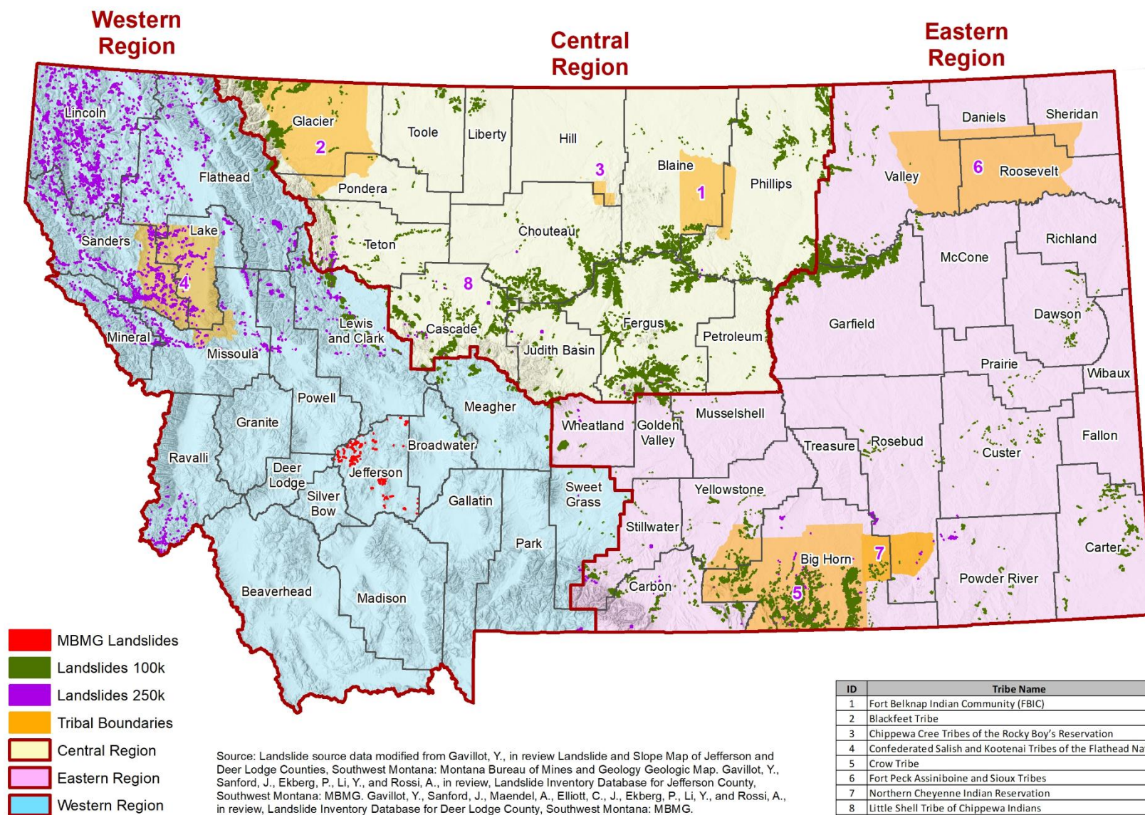
Figure 4-41 Montana Hazard Mitigation Planning Region Landslides
