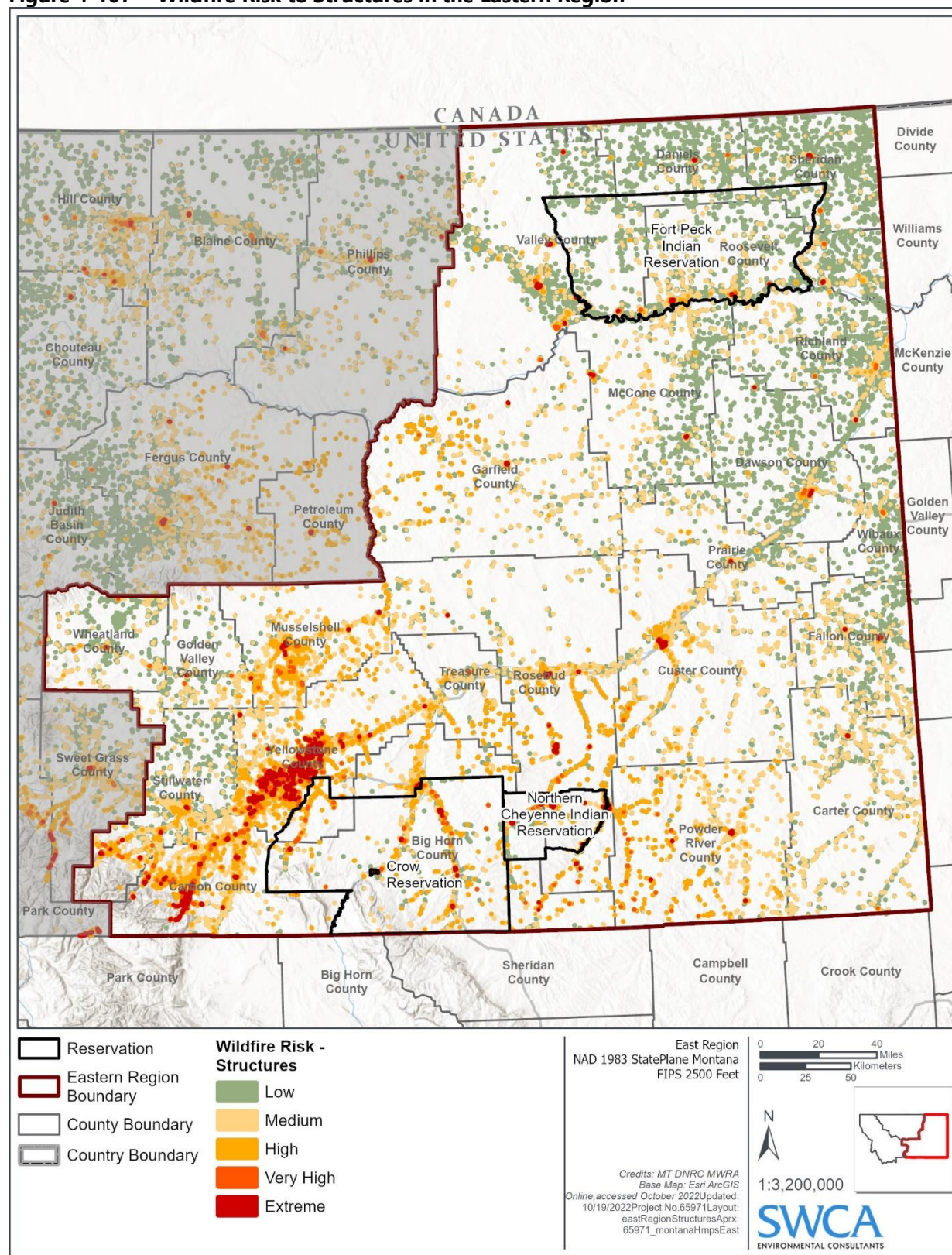
Figure 4-107 Wildfire Risk to Structures in the Eastern Region
