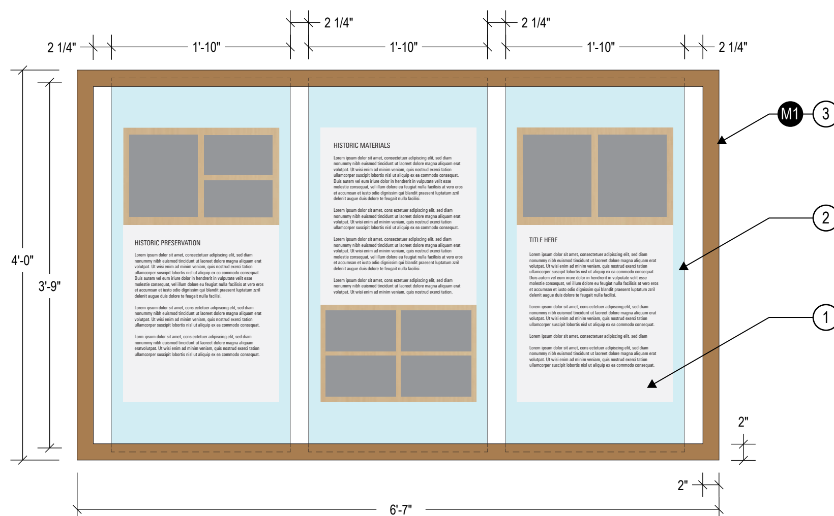
4 SIGN TYPE X-L1-3 - DETAIL ELEVATION 1" = 1'-0" NOTE: FPO CONTENT SHOWN, OWNER TO APPROVE FINAL CONTENT PRIOR TO FABRICATION
