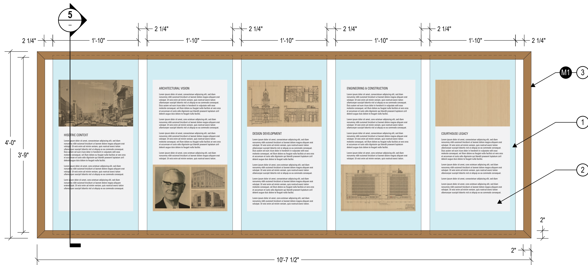
3 SIGN TYPE X-L1-1 - DETAIL ELEVATION 1" = 1'-0" NOTE: FPO CONTENT SHOWN, OWNER TO APPROVE FINAL CONTENT PRIOR TO FABRICATION
