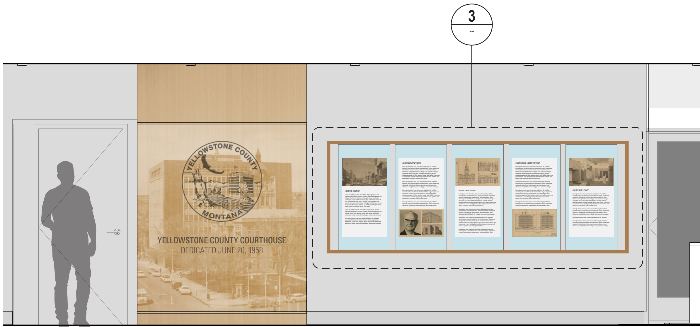
1 100 N LOBBY - N - SIGN TYPE X-L1-1 1/2" = 1'-0"
