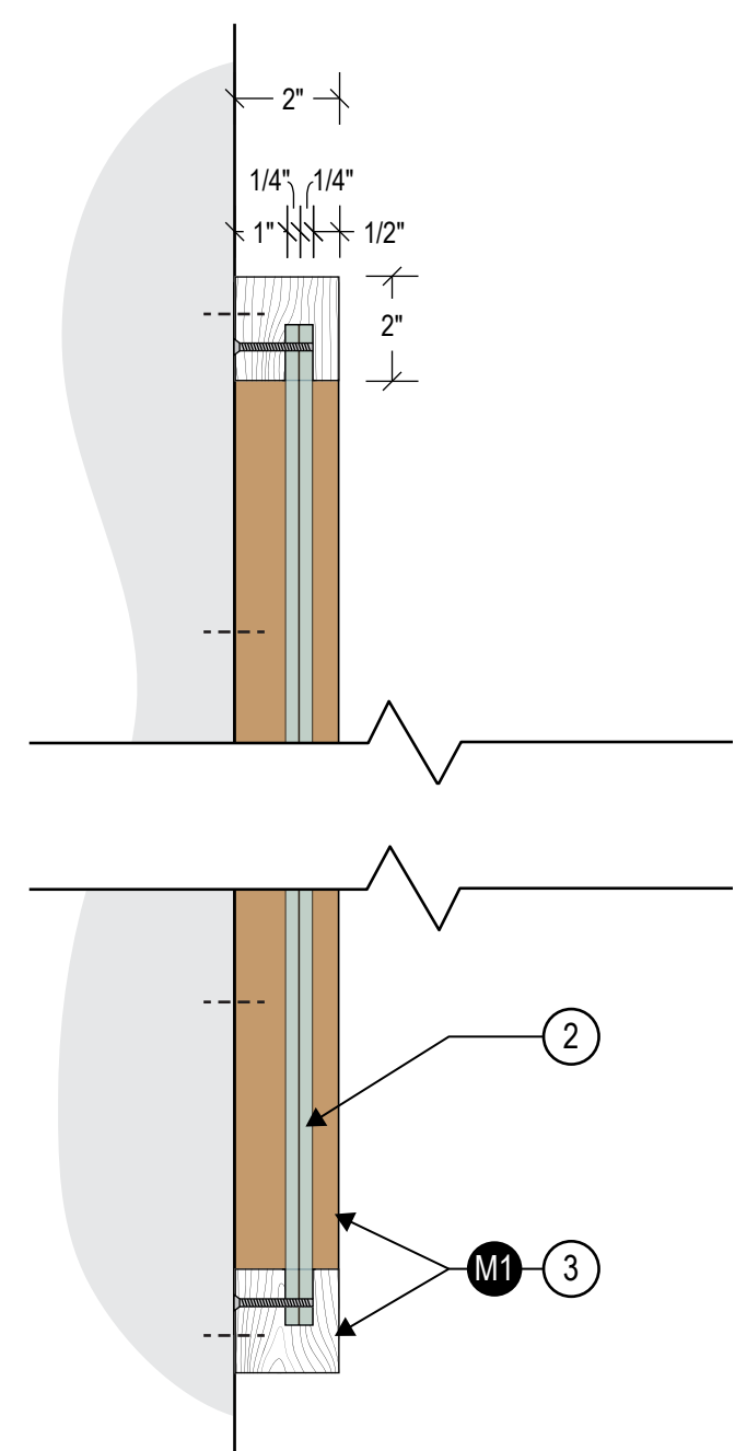
5 SIGN TYPE X - DETAIL SECTION (TYP.) 3" = 1'-0"
