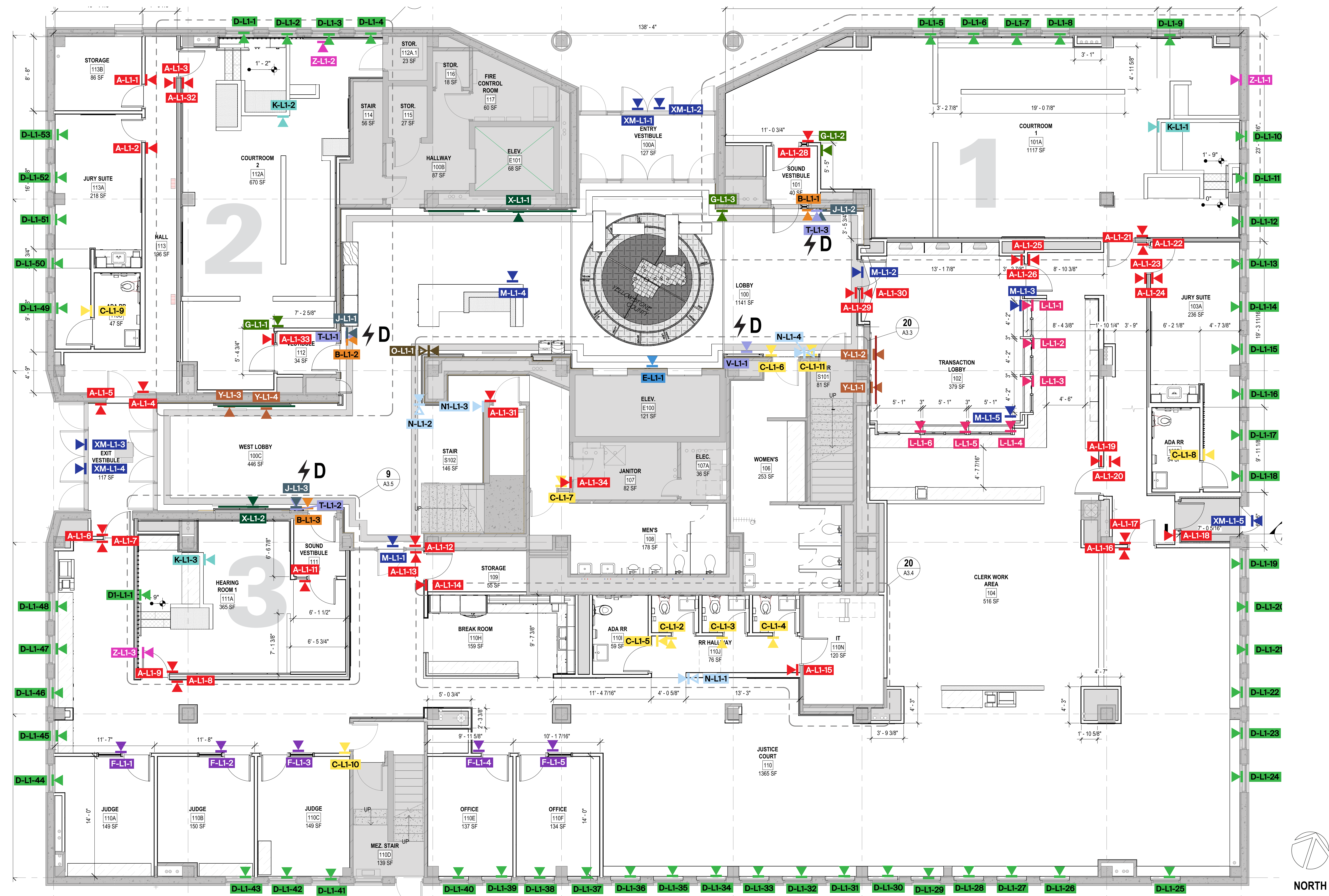
1 LEVEL 1 SIGNAGE LOCATION PLAN NTS
